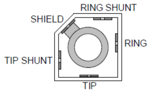
PIN LAYOUT (UNDERSIDE VIEW)
