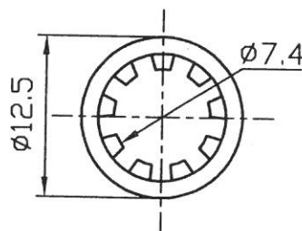
TEETH WASHER 1PC t=0.7
