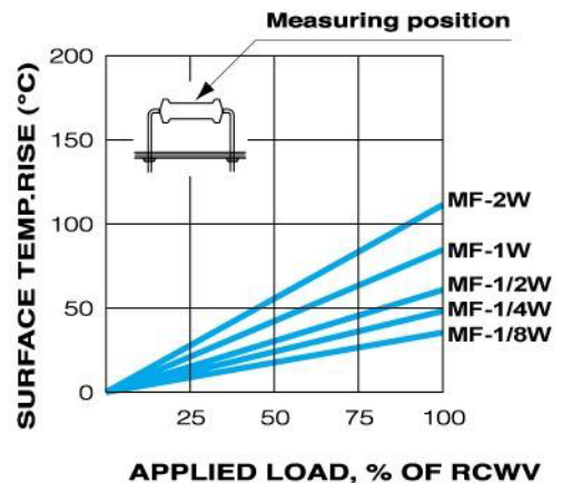
FIG.2 HOT-SPOT TEMPERATURE
