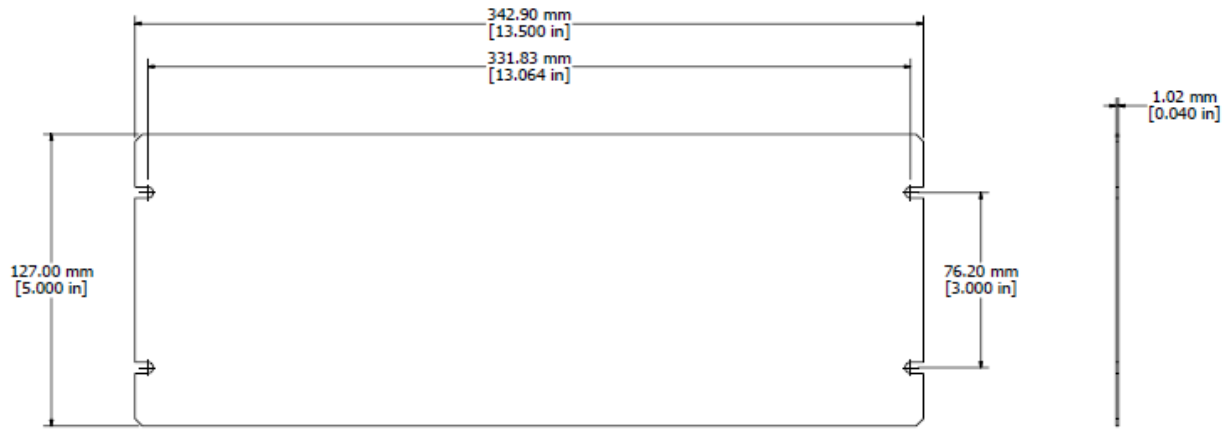
1434-18 - VIEW FROM TOP (SOLD SEPERATELY)
