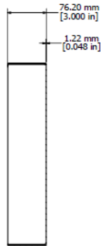
SECTION PP-PP
