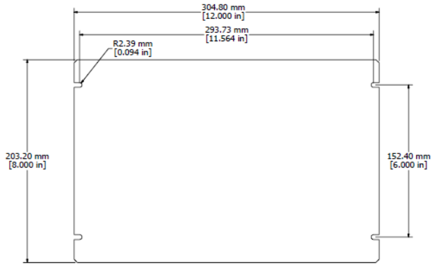
1431-22 OR 1431-22BK3 - VIEW FROM TOP (SOLD SEPERATELY)
