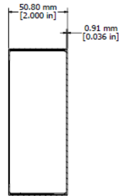
SECTION EE-EE
