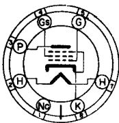
MEDIUM 7 PIN OCTAL BASE
