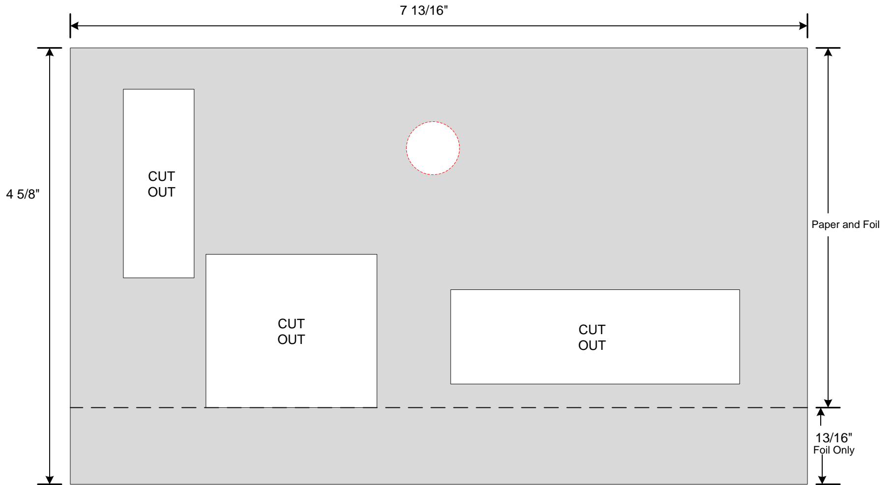
Foil Pattern
